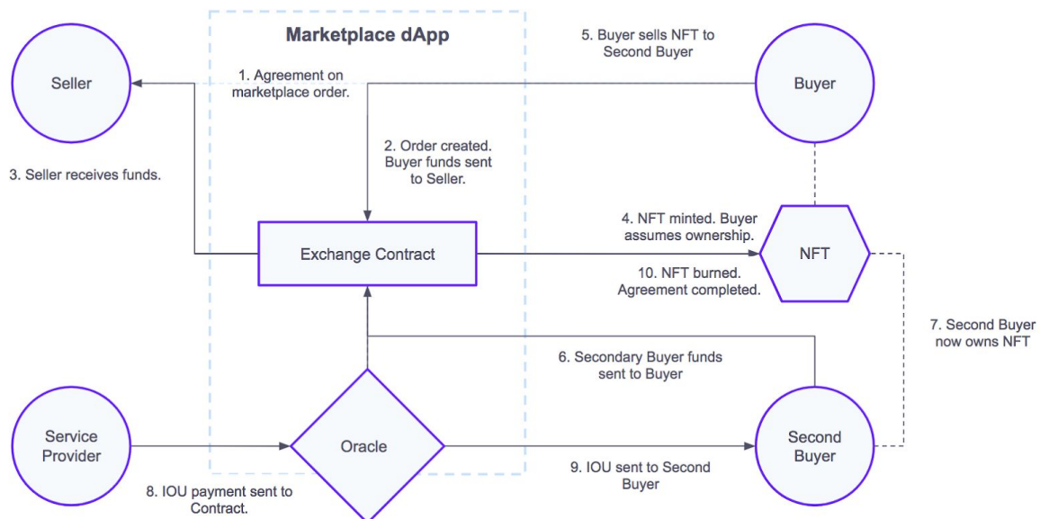
Figure 3.3.a: Example of an order execution sequence with a secondary taker scenario.
