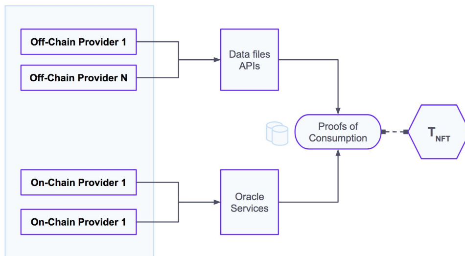
Figure 3.1.3.a: Visualization of sourcing Proofs of Consumption from off-chain and on-chain suppliers
